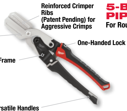
REINFORCED CRIMPER RIBS
