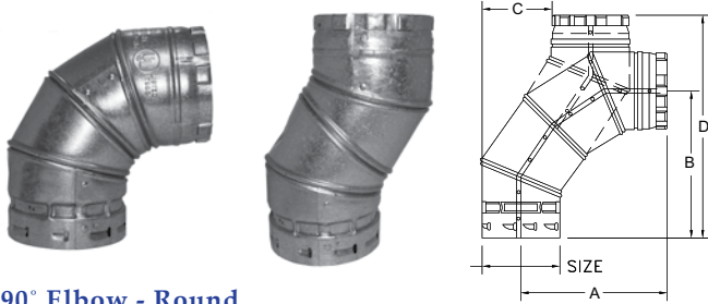
90° Elbow - Round
