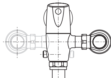
VALVE LEFT or RIGHT HAND INSTALLATION
