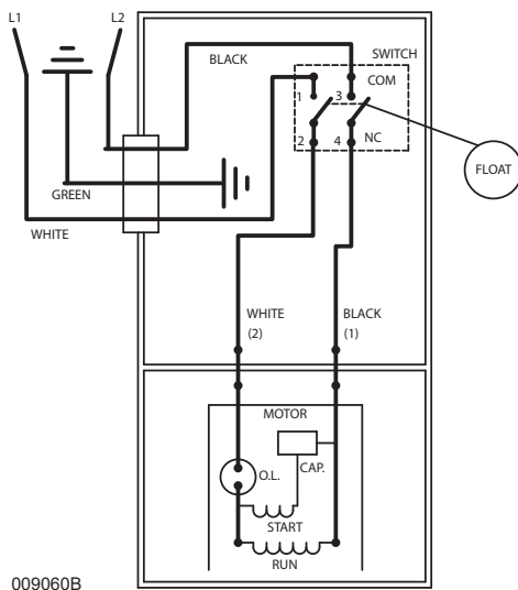
009060B WIRING DIAGRAM FOR MODELS "M98-"All revisions" "D98-"All revisions" 11/90 thru Current
