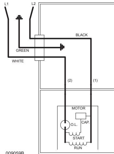
009059B WIRING DIAGRAM FOR MODELS "N98-"All revisions" "E98-"All revisions" 11/90 thru Current
