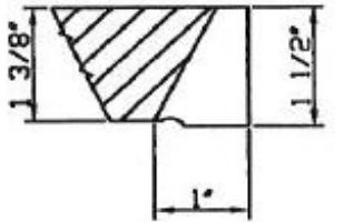
SECTION OF COVER THRU. RECESS
