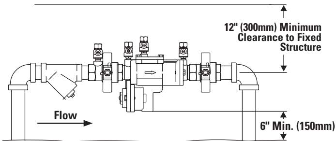
Series LF860 1/2" - 2" Outdoor Installation
