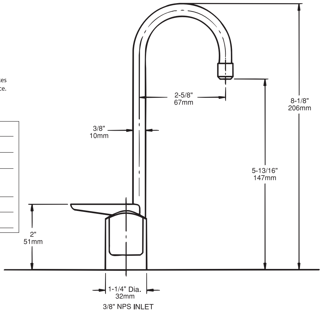
SIDE VIEW
