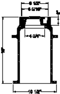
VB101 Weight: 55 lbs.
