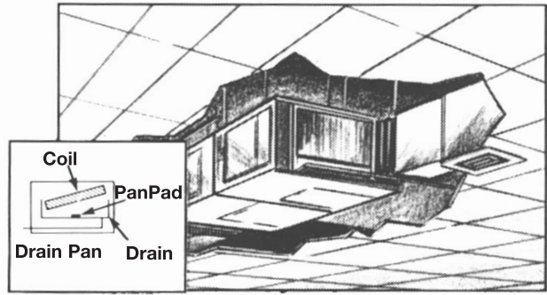
Ceiling Units
