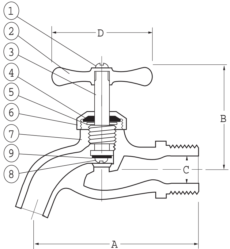
Pictured Model T-532CP Cut-away
