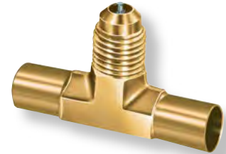
A31234 1/4" ODS x 3/8" ODF Brass Tee
