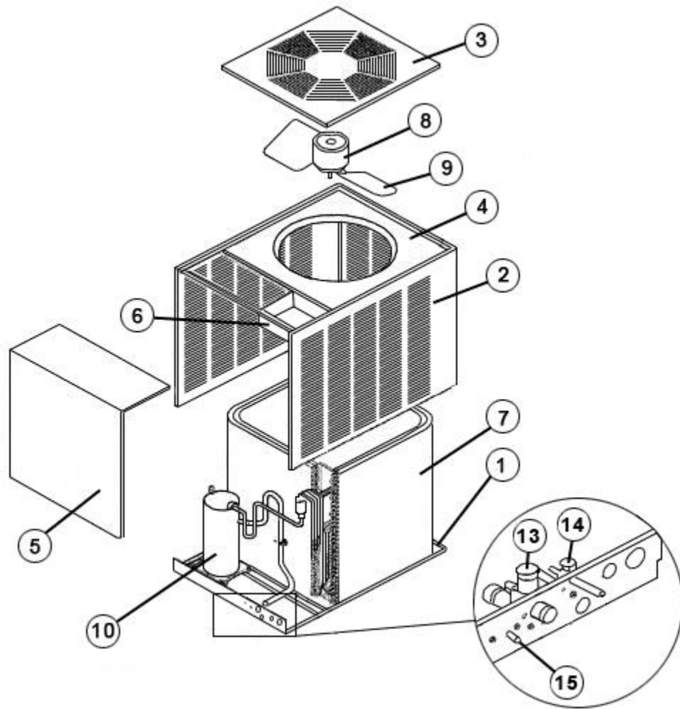
Exploded View
