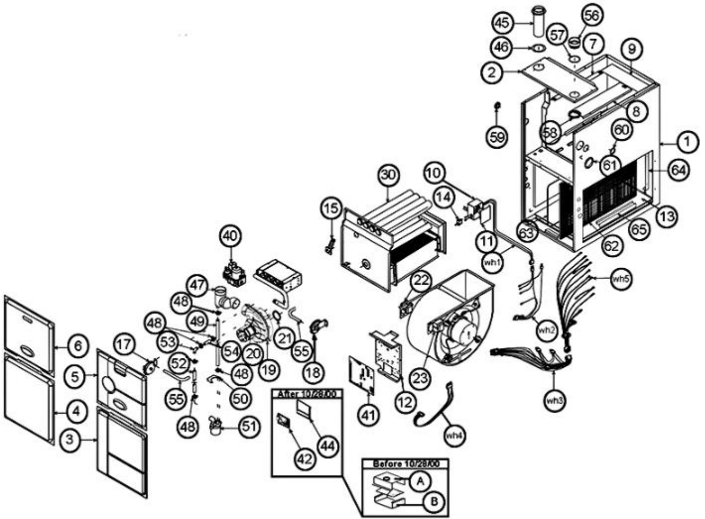
Exploded View
